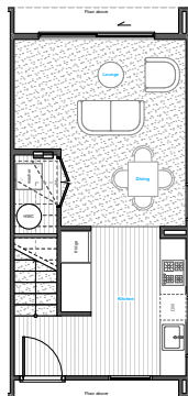
GROUND FLOOR
